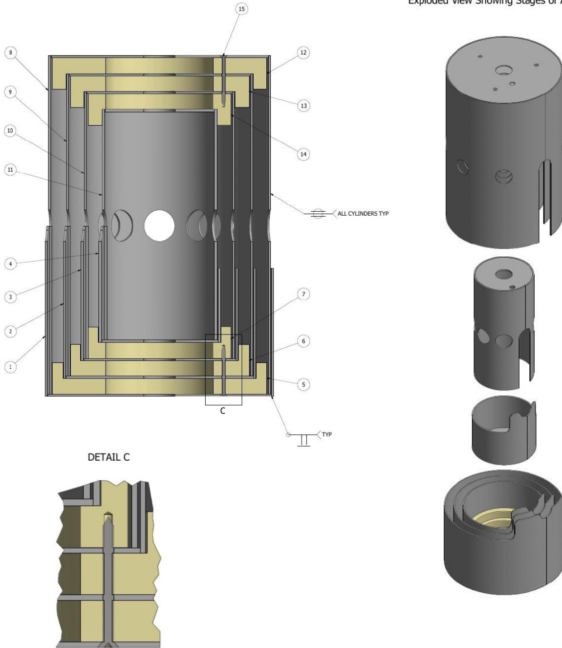
Exploded View Showing Stages of Assembly
